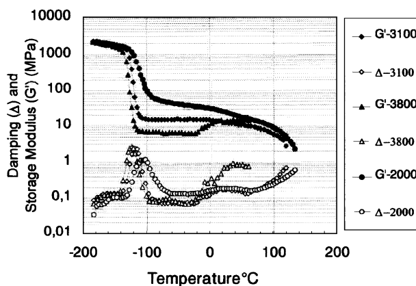
Fig. 4. Dynamic-mechanical spectra ( G' and \Delta vs T ) for samples of S1 series.
